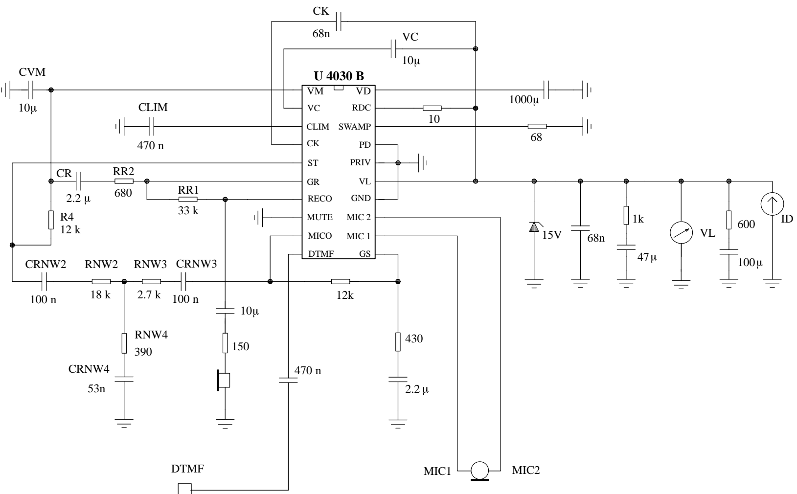
Figure 9. Application Circuit
